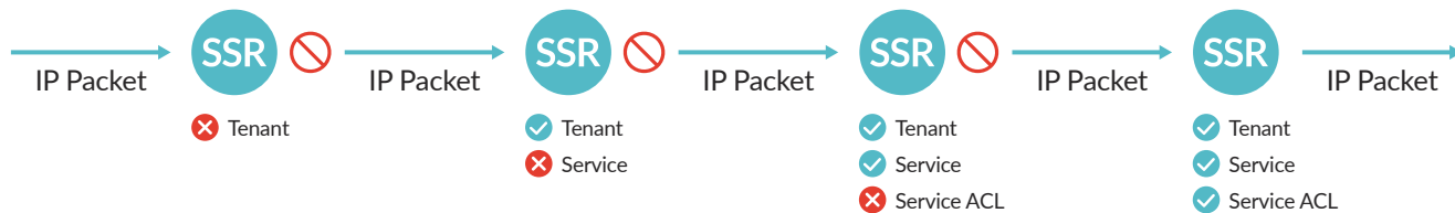
Figure 2: Deny-by-default policy
