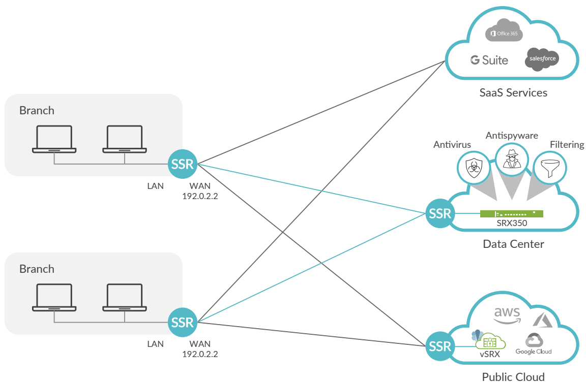
Figure 3: For NGFW treatment, the Session Smart Router can be used with the Juniper SRX.
